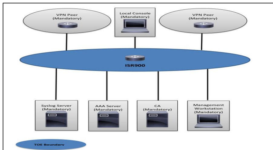
Figure 1: TOE Architecture
